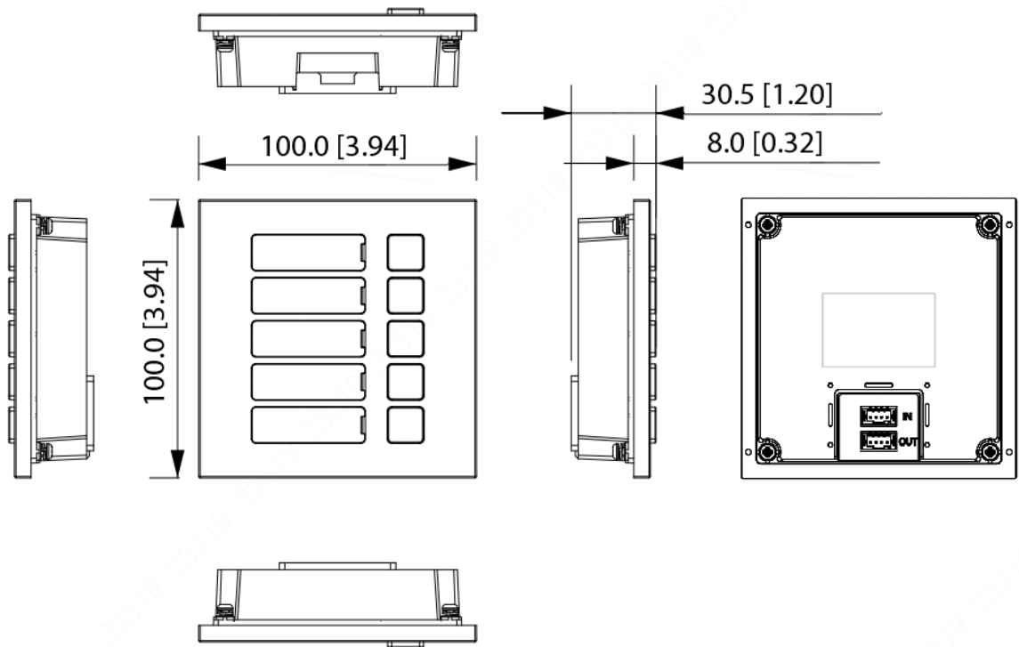
Figure 3-1 Dimensions (unit: mm [inch])
