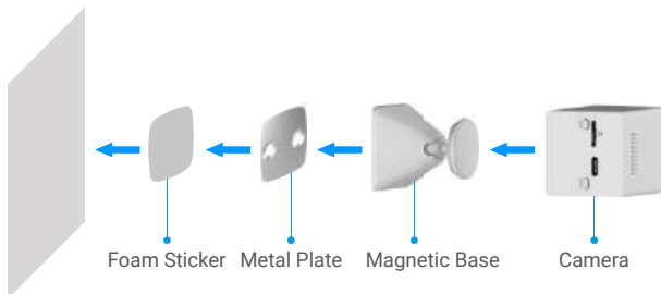
Fig.1 Mount by Foam Sticker
