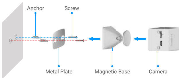
Fig.2 Mount by Screws
