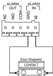
Figure 3-3 Door Magnetic Wiring
