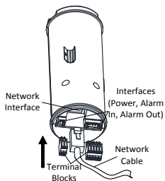
Figure 4-3 Insert Terminals and Network Cable
