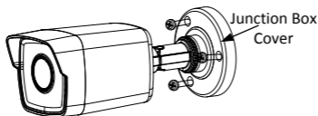
Figure 2-5 Fix the Camera on Junction Box's Cover
