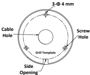
Figure 2-1 The Drill Template
