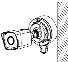
Figure 2-7 Combine Junction Box's Cover with its Body
